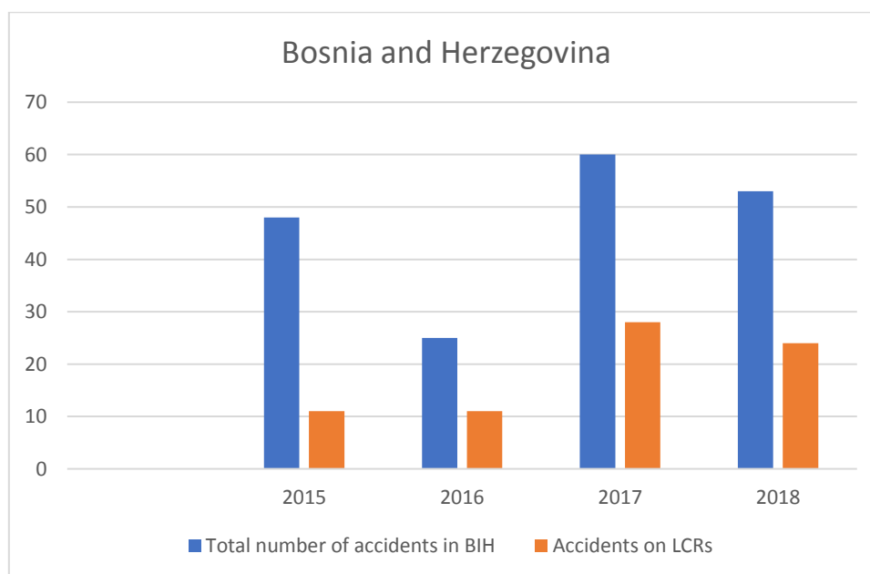
Figure 5: Comparison between the total number of accidents and those on LCRs in BiH, for the period 2015-2018
