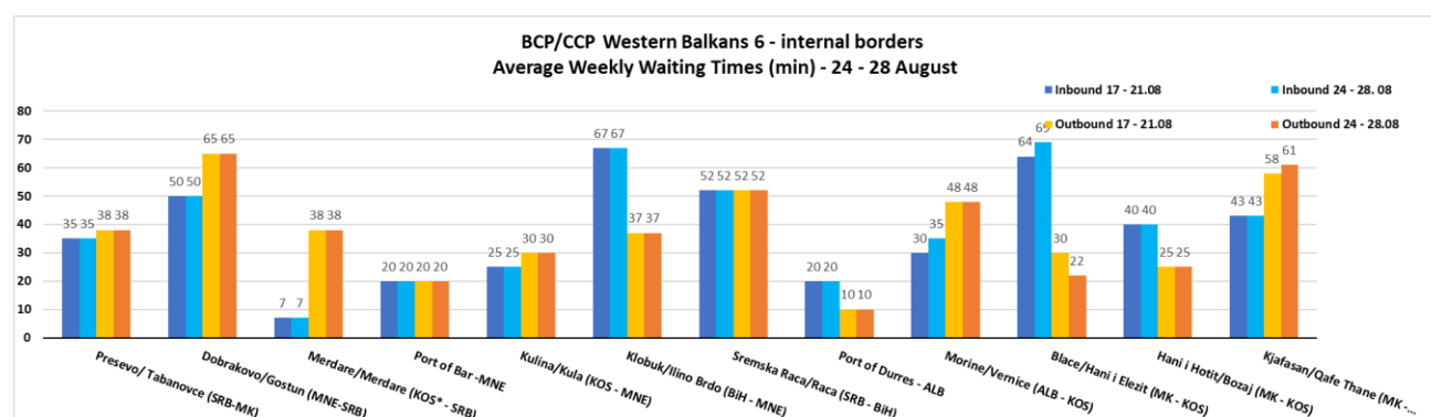
Figure 1: Average weekly waiting times (consecutive weekly trends)
